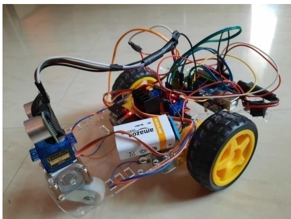
Surveillance robot developed by the students
