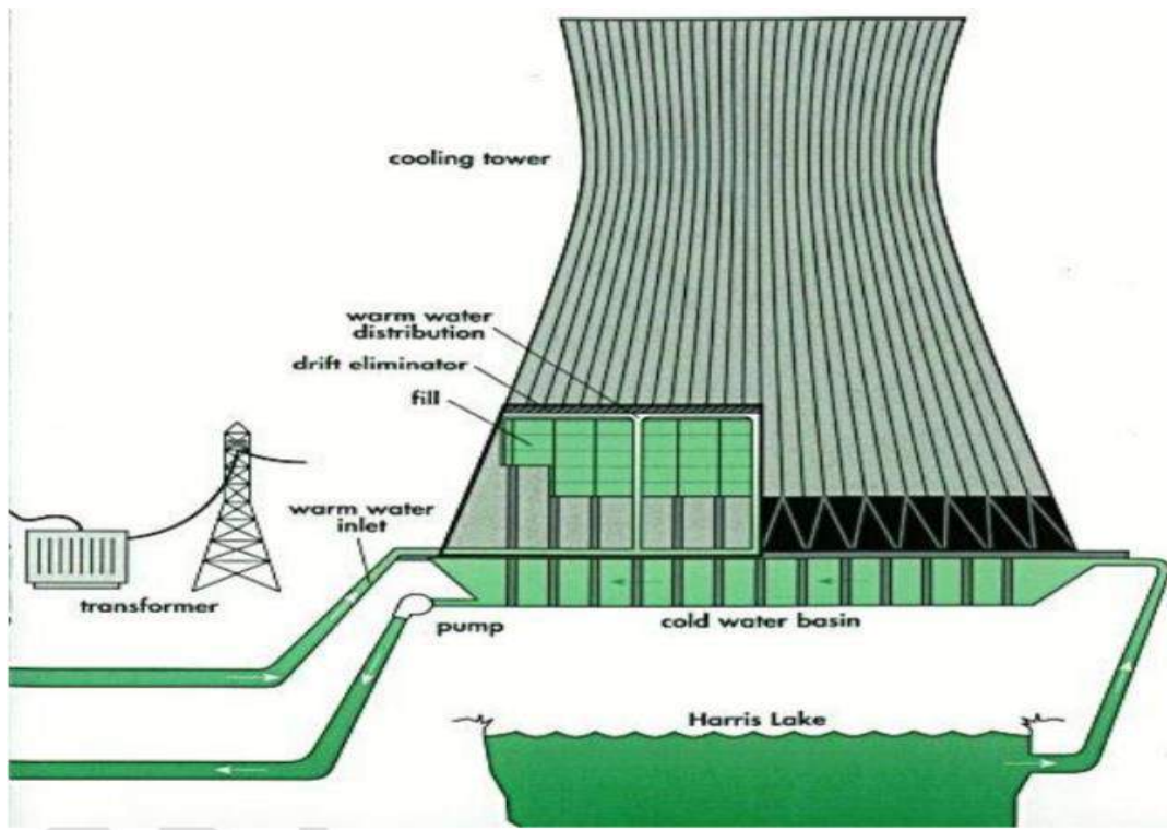
Figure 1.5 cooling tower
