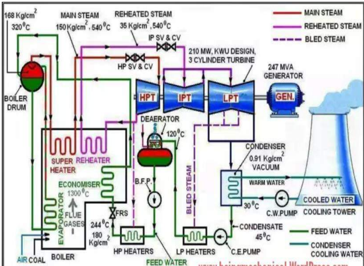
Figure.1.3 Typical Working Layout of Thermal Power Plant
