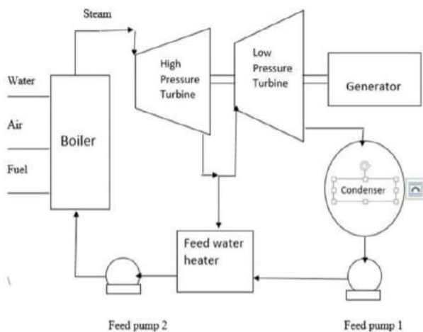
Figure 1.2. Plant Model
